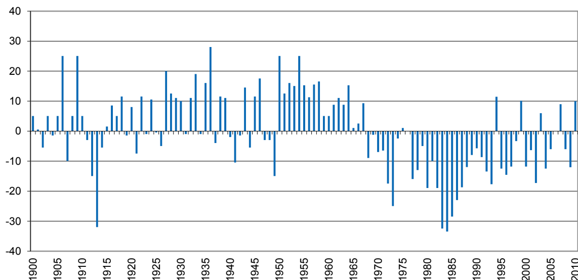
Figure 1 : Evolution de l’indice standardisé des précipitations (ISP) sur le bassin du Niger à Niamey de 1900 à 2012. Evolution of the Standard Precipitation Index (SPI) of the Niger River Basin at the Niamey station, from 1900 to 2012; SPI is calculated as: SPI = (P_i - P_{mean}) / \sigma , with P_i = Precipitation value for year i ; P_{mean} = mean rainfall of the series; \sigma = standard deviation of the series; adimensional index.
