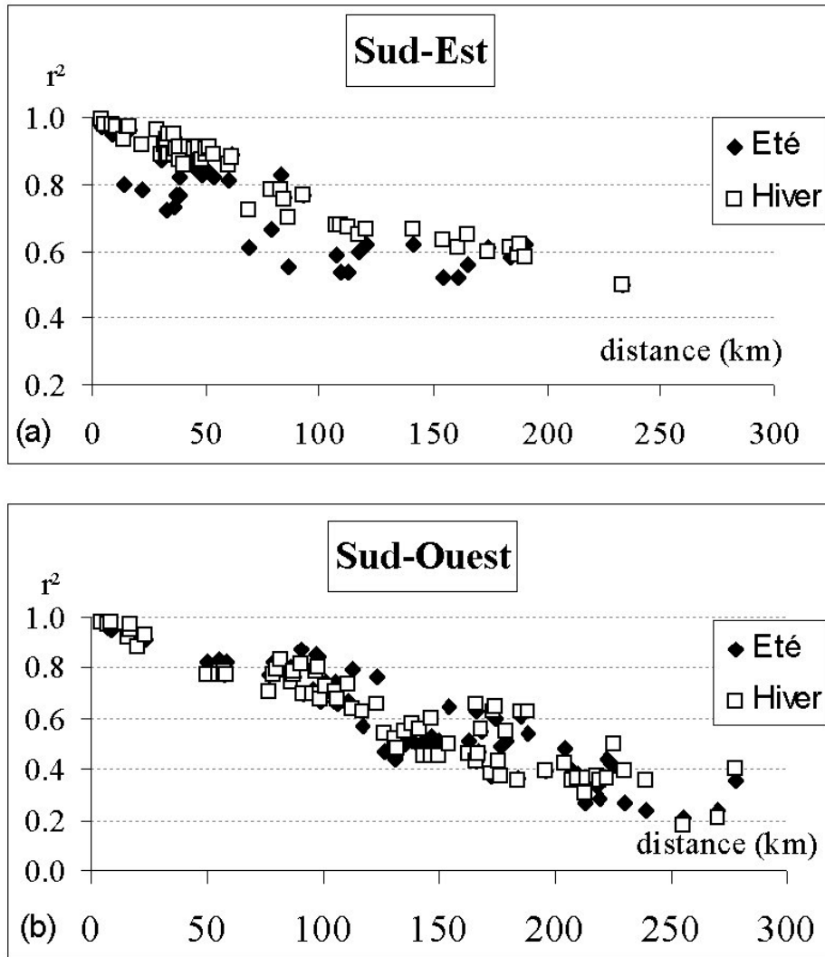
Figure 3 : Régionalisation et effet saisonnier des corrélations dans le Sud-Est (a) et le Sud-Ouest (b). Regionalization and seasonal effect of the correlations in South-East (a) and South-West (b).
